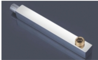
SS Shower Arm SQUARE with Brass Bush DG-ESS-150 | 9" - 225mm DG-ESS-151 | 12" - 300mm DG-ESS-152 | 18" - 450mm DG-ESS-153 | 24" - 600mm
