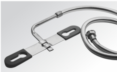
Jet Spray FLAT (Full Set) DG-ESS-04 | 1 MTR DG-ESS-05 | 1.5 MTR Material : AISI SS-304
